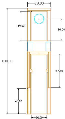
VISTA FRONTAL
